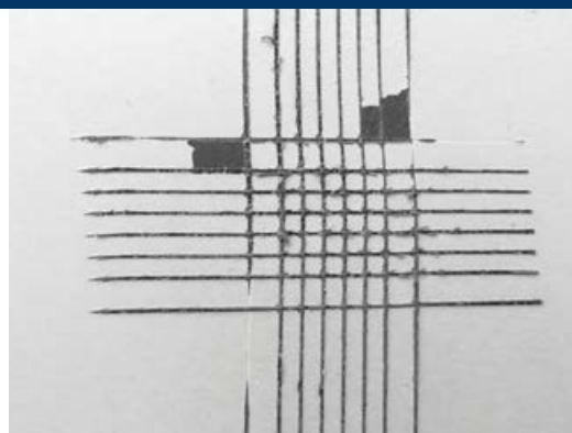
Ultrafill 2 – good performance on PP + EDPM without pre-treatment
