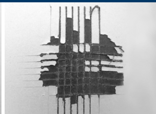
Standard product – low performance on PP + EDPM without pre-treatment
